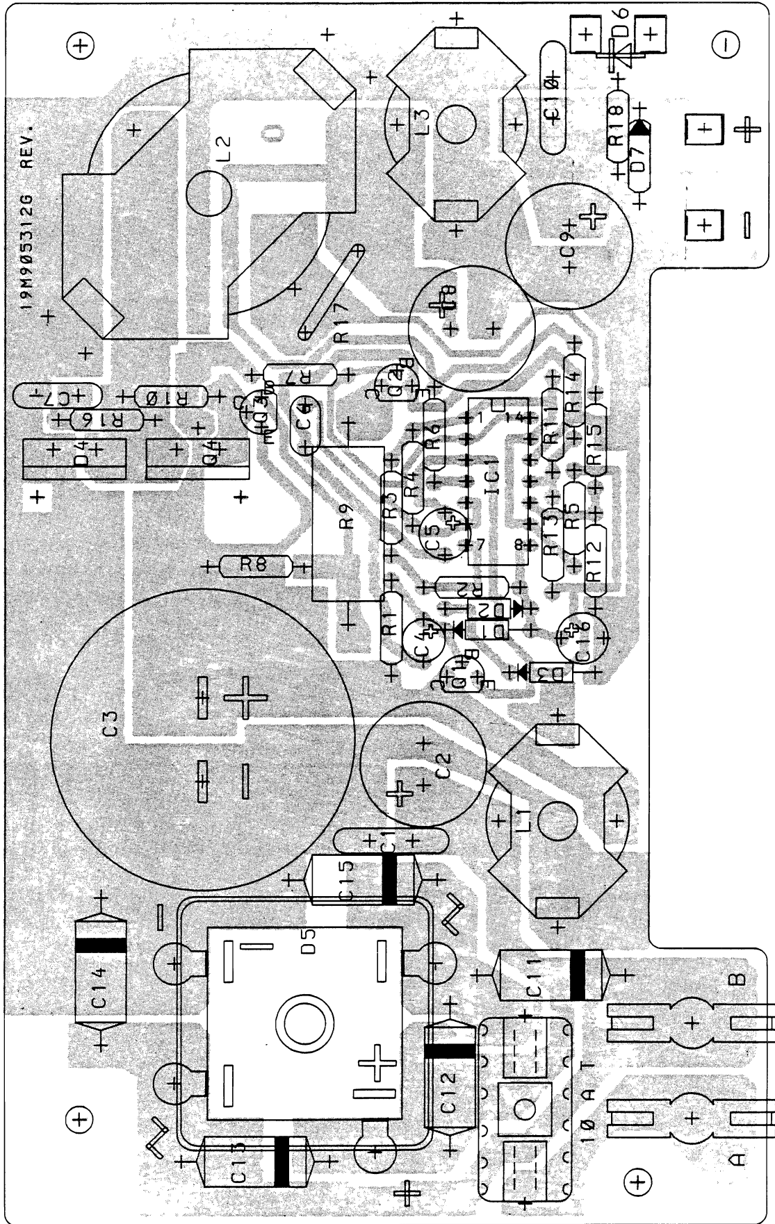
POWER SUPPLY C9PS04 COMPONENT LAYOUT
