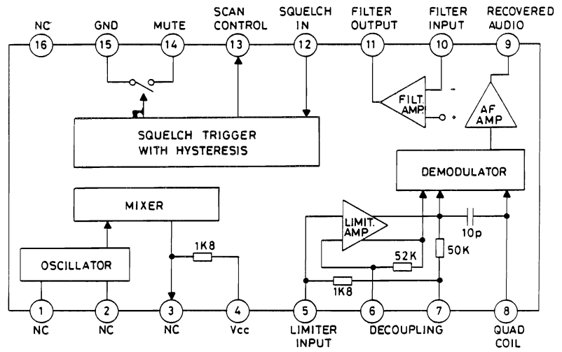
BLOCK DIAGRAM FOR U401
